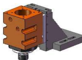
80-ER 立装+两槽支架 80-ER Vertical Installation + Two-slot Bracket
